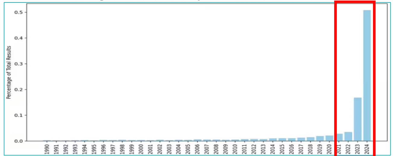
Percentage of PubMed Search Query "delve" Results (1990 - 2024)
